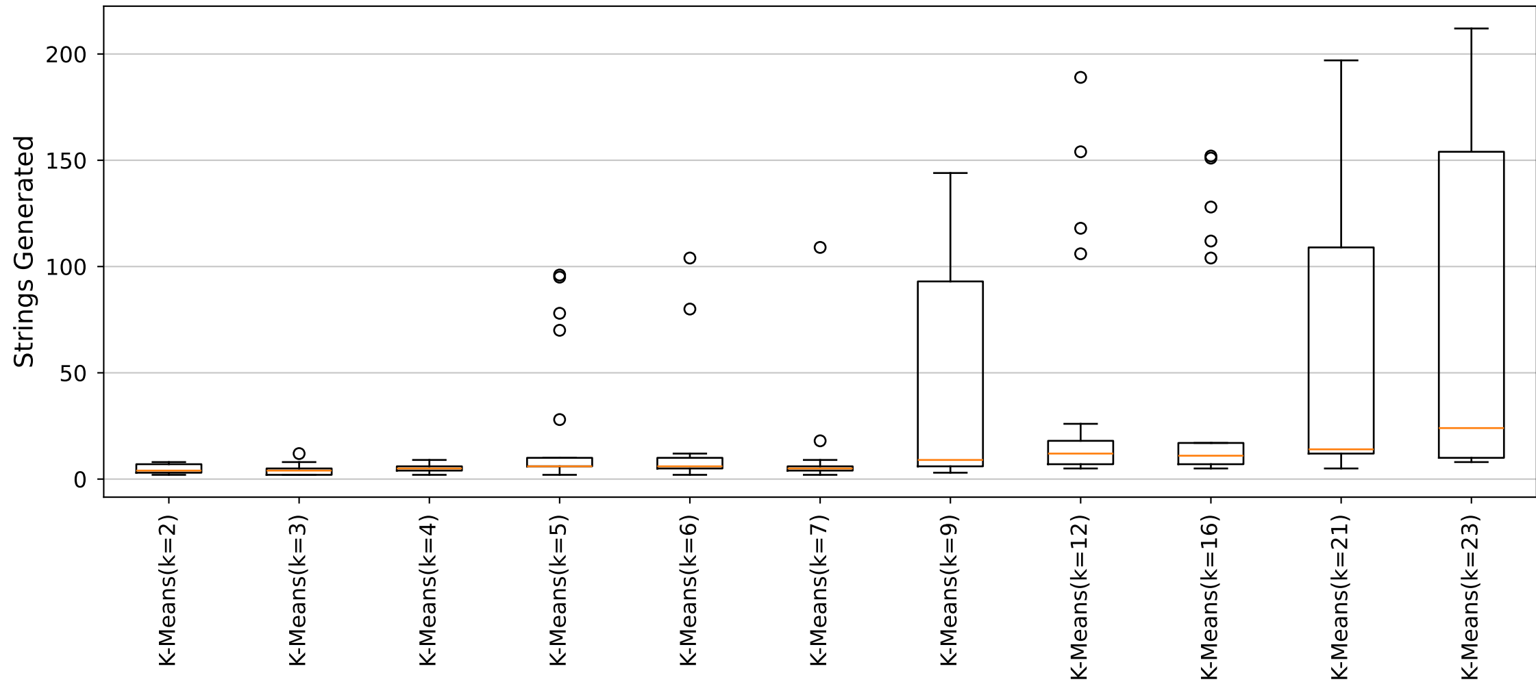
YARA Rules Strings Generated Distribution (Cluster5_Size23 dataset)
